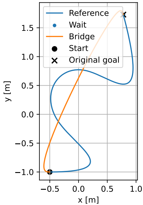
Bridged Pololu Reference
